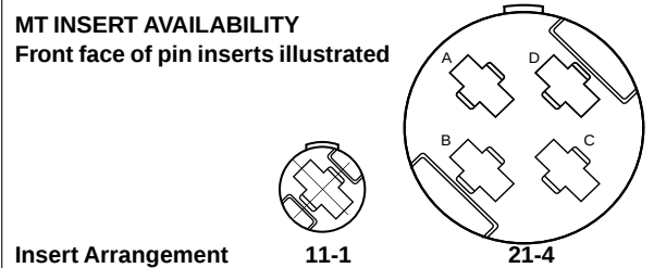
MT38999 Connectors
