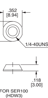
DRESS NUT
