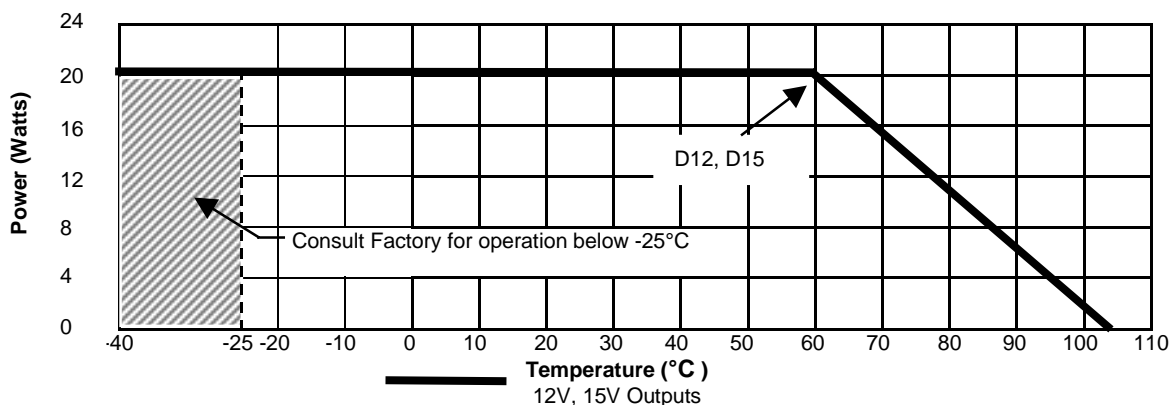
Total Output Power vs. Ambient Operating Temperature
