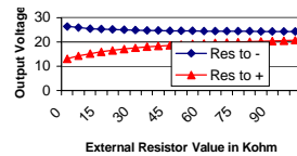
PM2048D12 Voltage Trim Adjusts the total voltage (+) out to (-) out
