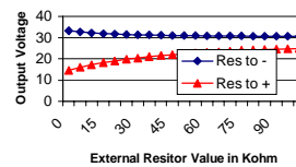
PM2048D15 Voltage Trim Adjusts the total voltage (+) out to (-) out
