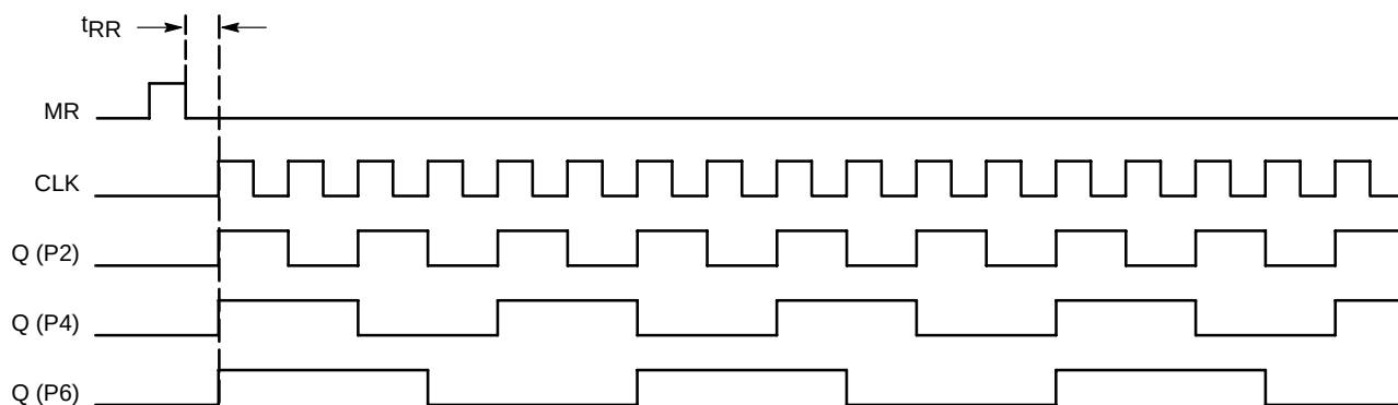
Figure 3. Timing Diagram
