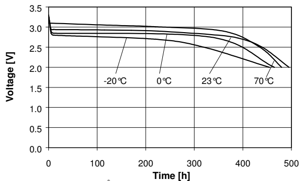
Temperature performance Load 47kΩ
