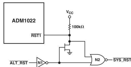
Figure 10. Separation of \overline{\text{RST1}} Input from \overline{\text{RST1}} Output
