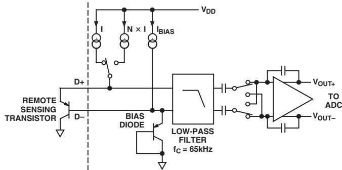
Figure 3. Signal Conditioning
