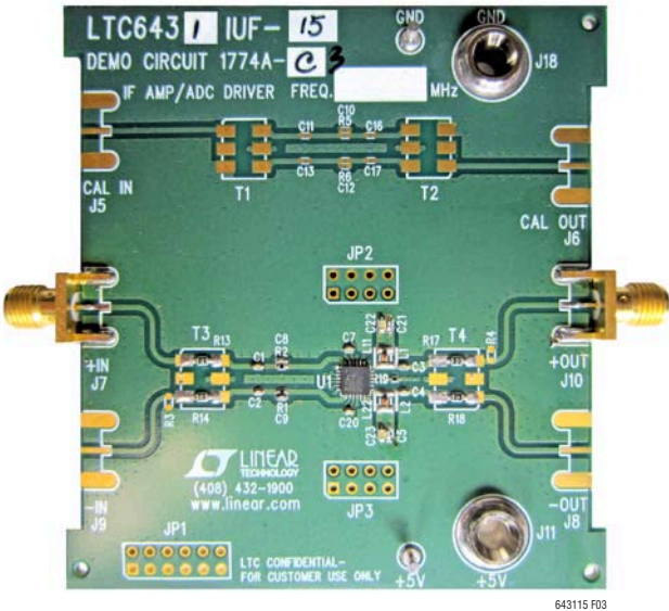
Figure 3. Demo Board
