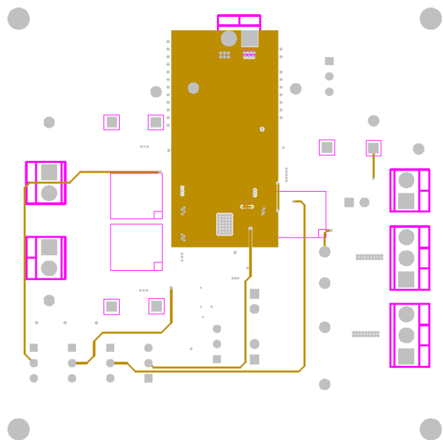
Figure 5. Board Layout (Middle 3 rd ) Layer
