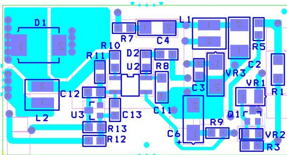
Figure 4 - Bottom Side, SMT Printed Circuit Layout (Top View).
