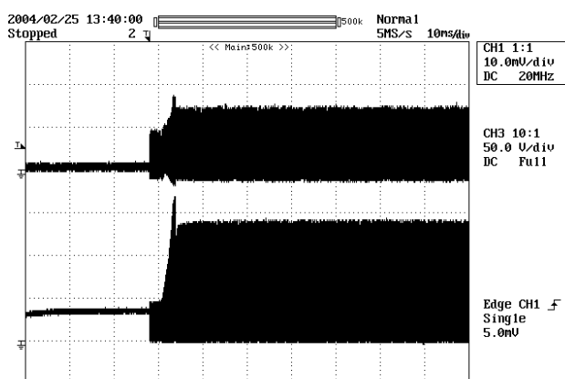
Figure 15 – 36 VDC Input, 2 A Resistive Load.
