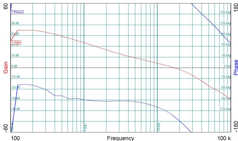
Figure 27 - Gain-Phase Plot, 57 VDC, Light Load (100 mA). Vertical Scale: Gain = 10 dB / div, Phase = 30° / div. Crossover Frequency = 10.8 kHz, Phase Margin = 40°
