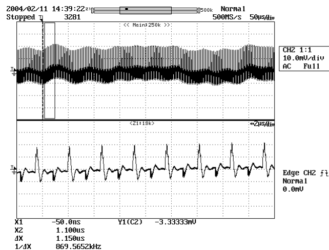
Figure 22 - Ripple, 48 VDC, Full Load. Top: 10 mV / div, 50 μs / div. Bottom: 10 mV / div, 2 μs / div.
