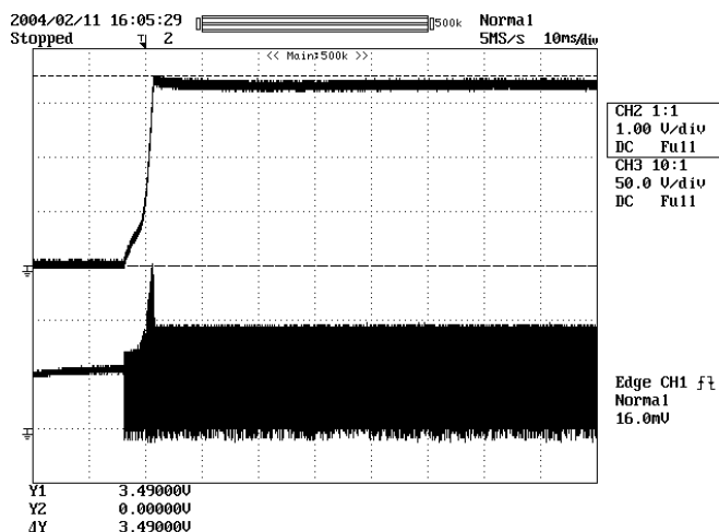
Figure 14 - Start-Up Profile, 57 VDC, No Load (worst-case).
