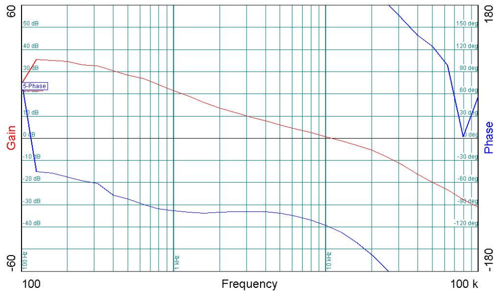
Figure 25 - Gain-Phase Plot, 36 VDC, Maximum Load (2 A). Vertical Scale: Gain = 10 dB / div, Phase = 30° / div. Crossover Frequency = 10.0 kHz, Phase Margin = 60°
