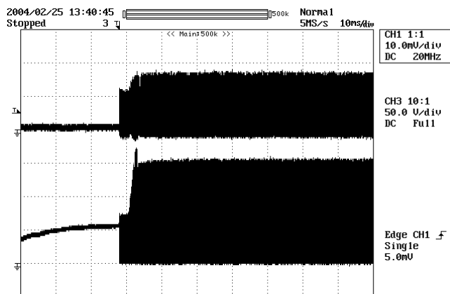
Figure 16 – 57 VDC Input, 2 A Resistive Load.
