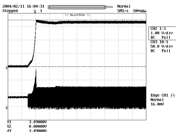
Figure 13 - Start-Up Profile, 36 VDC, No Load (worst-case).
