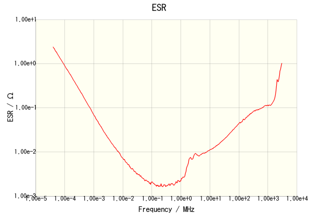
C3225X5R0J226K200AA
