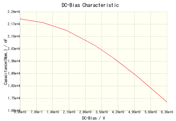
C3225X5R0J226K200AA
