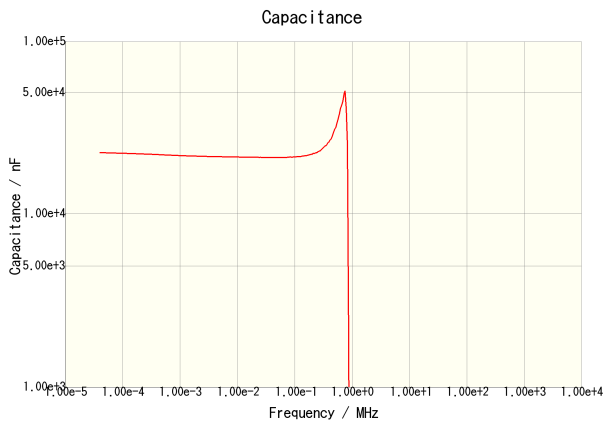
C3225X5R0J226K200AA
