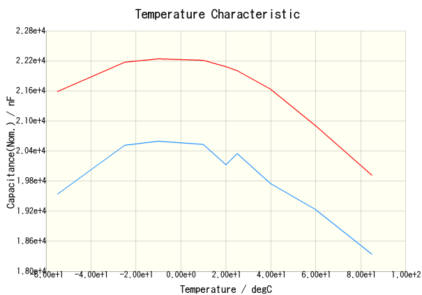
C3225X5R0J226K200AA(DC Bias = 0V) C3225X5R0J226K200AA(DC Bias = 3.15V)
