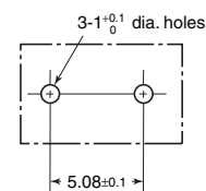
<PCB Mounting Dimensions (Reference)>
