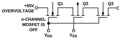
Figure 12. +55 V Overvoltage Input to the ON Channel
