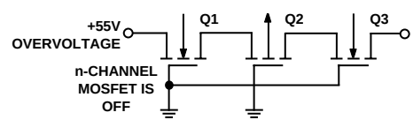
Figure 14. +55 V Overvoltage with Power OFF
