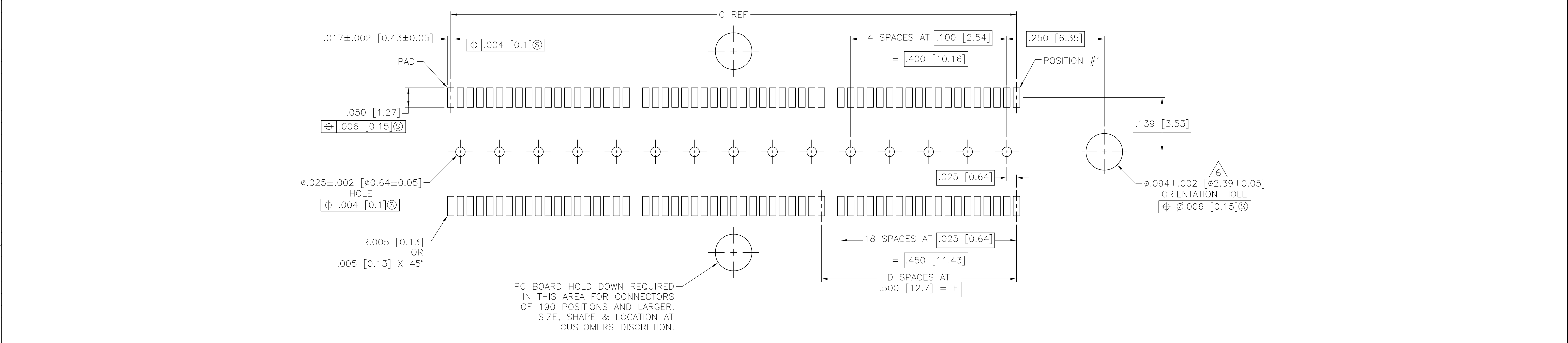
RECOMMENDED PC BOARD LAYOUT (VIEWED FROM CONNECTOR SIDE)
