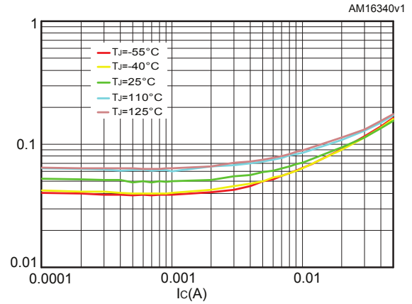
Figure 2. V_{CE(sat)} @ h_{FE} = 10
