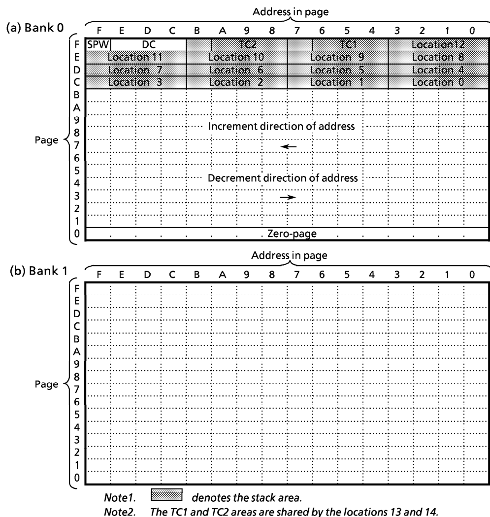
Figure 2-6. Data Memory Map
