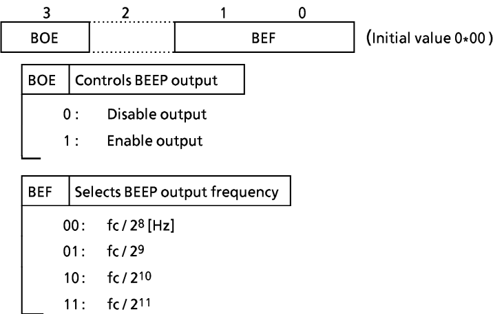
Figure 3-39. BEEP Output Control Command Register
