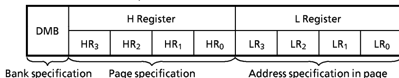
Figure 2-4. Configuration of H, L registers and DMB
