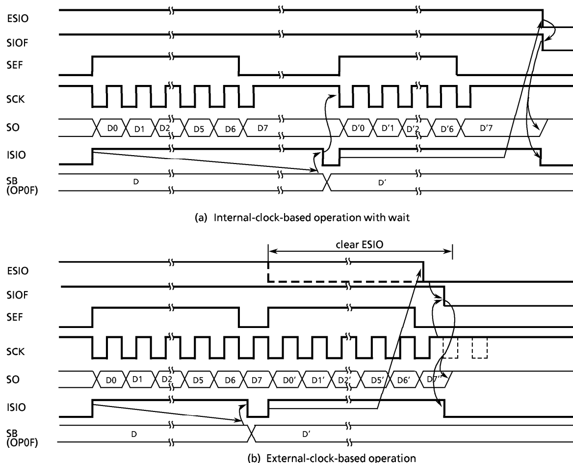
Figure 3-43. Transmit Mode
