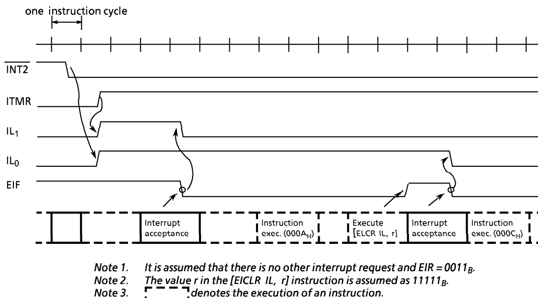
Figure 2-29. Interrupt Timing Chart (Example)
