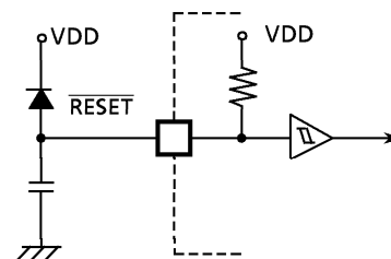
Figure 2-30. Simplified power-on-reset circuit
