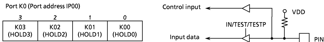
Figure 3-3. Port K0
