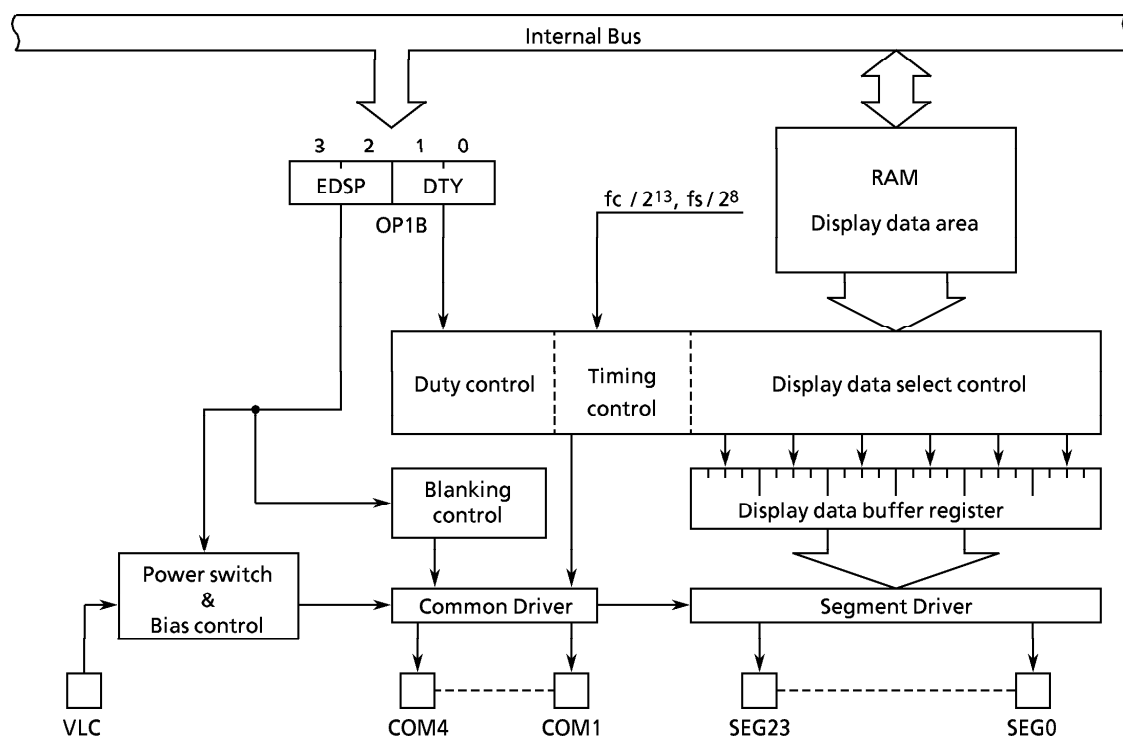
Figure 3-22. Configuration of LCD Driver
