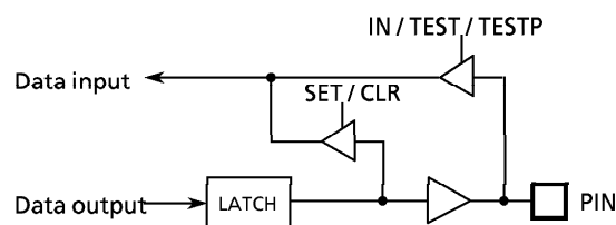
Figure 3-6. Port R6
