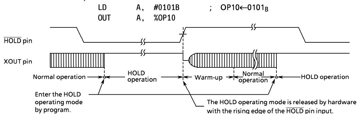
Figure 2-27. Edge-sensitive Release Mode
