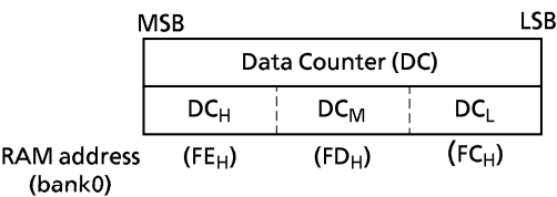
Figure 2-7. Data Counter
