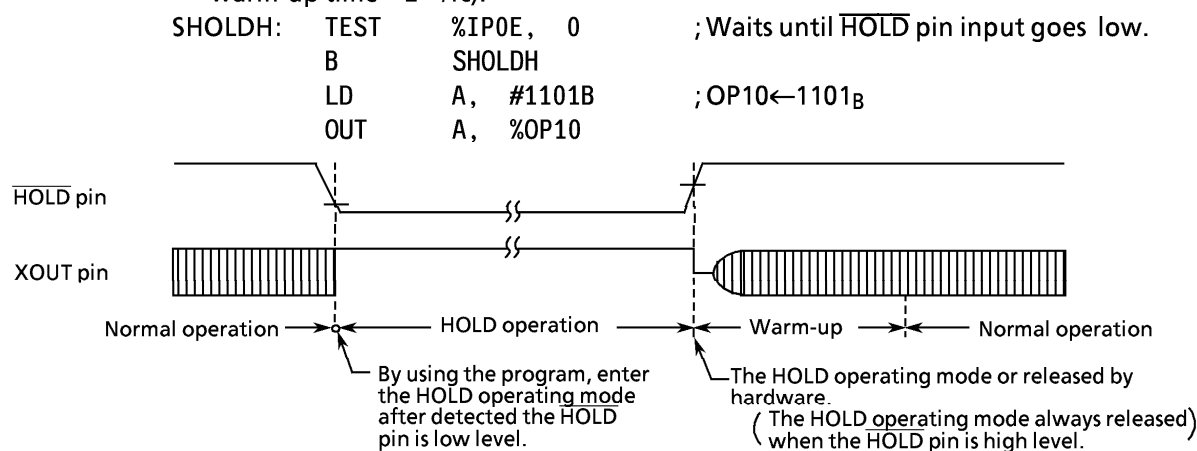
Figure 2-26. Level-sensitive Release Mode
