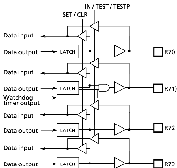
Figure 3-7. Port R7
