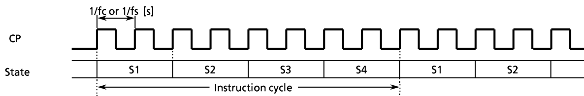
Figure 2-22. Instruction Cycle
