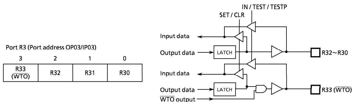
Figure 3-4. Port R3
