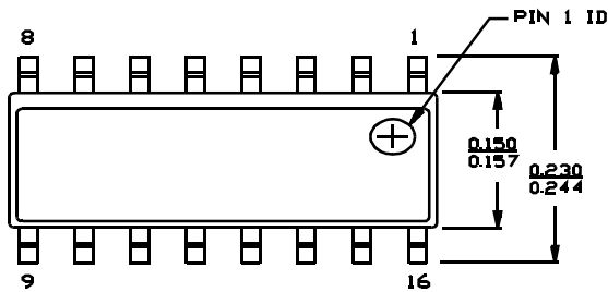
16-lead (150-mil) Molded SOIC S16
