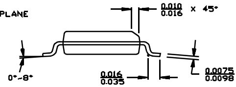
16-lead Thin Shrink Small Outline Package (4.40 MM Body) Z16
