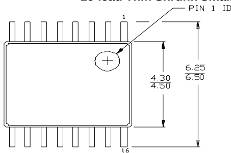
16-lead Thin Shrink Small Outline Package (4.40 MM Body) Z16
