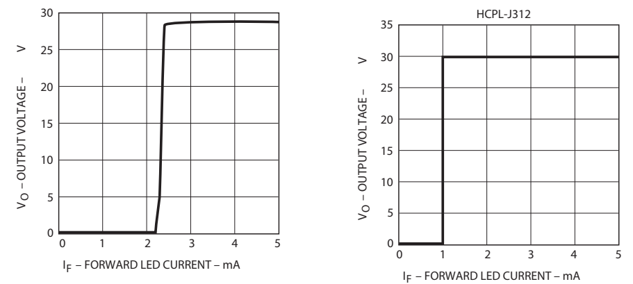
Figure 15 Transfer Characteristics
