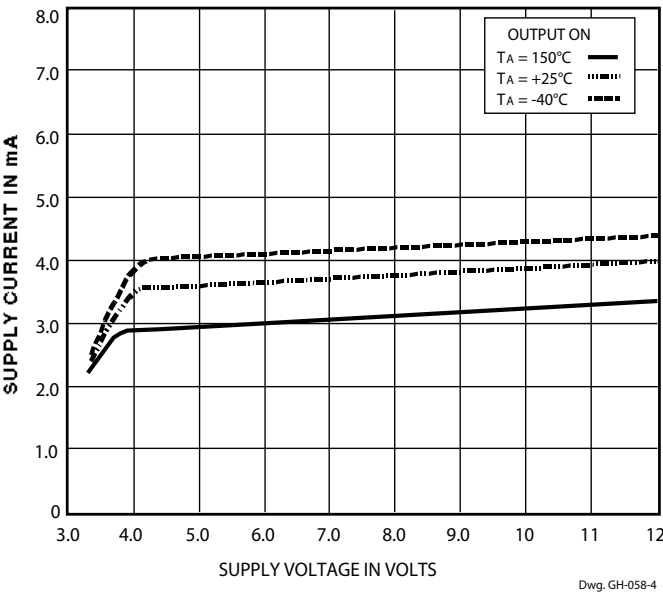
SUPPLY CURRENT
