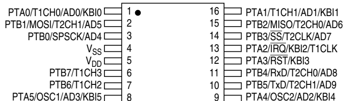
16-PIN ASSIGNMENT MC68HC908QCxx TSSOP
