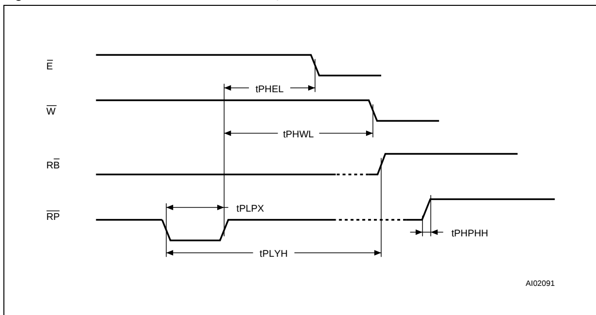
Figure 9. Read and Write AC Characteristics, \overline{R} Related
