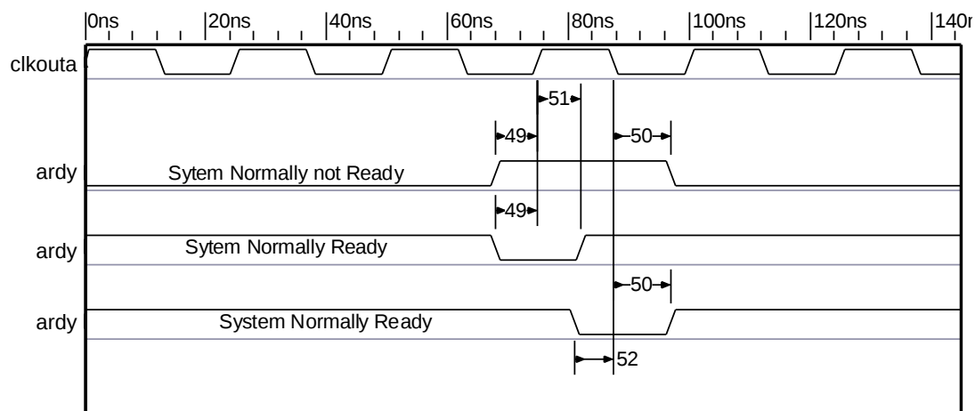
Figure 23. ardy—Asynchronous Ready
