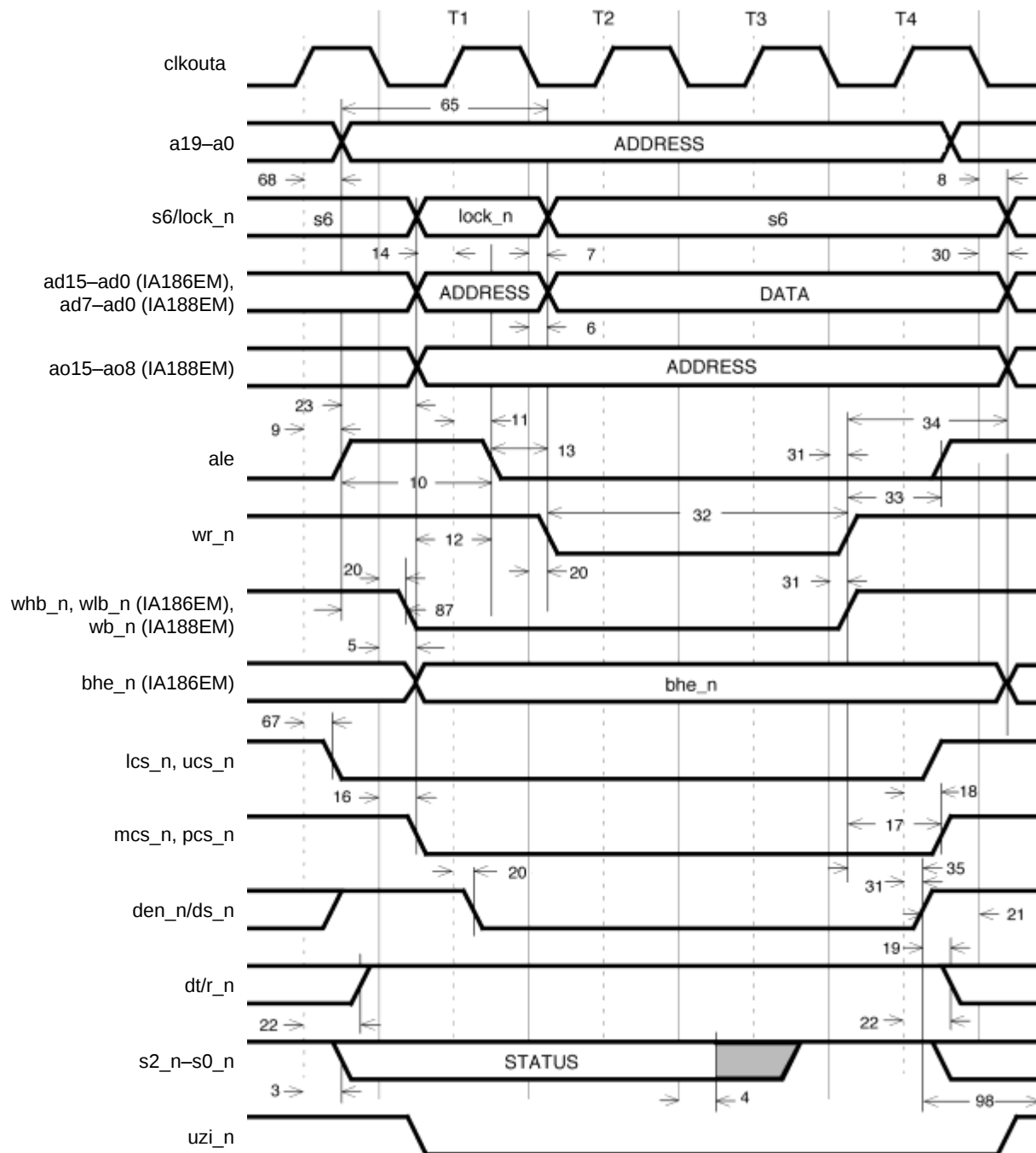
Figure 13. Write Cycle
