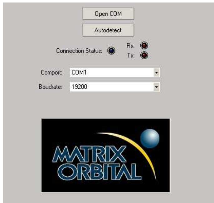
Figure 12: uProject Settings
