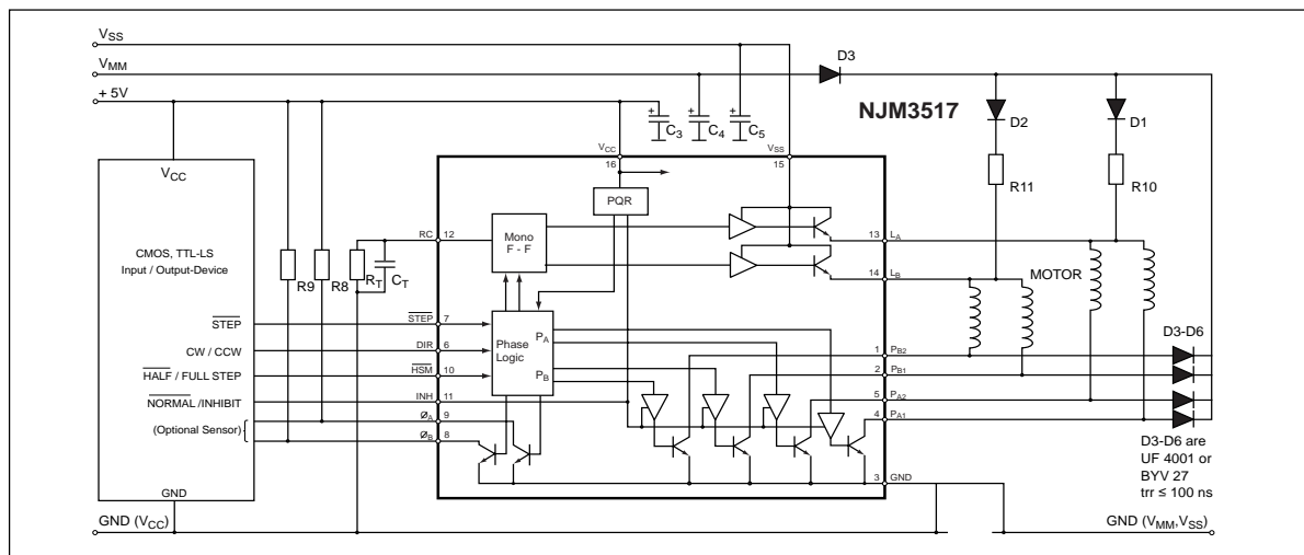
Figure 3. Typical application
