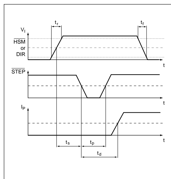
Figure 6. Timing diagram
