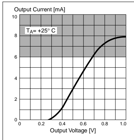
Figure 15. Typical I_O vs. V_{OCE\text{ Sat}} "Zero output" saturation
