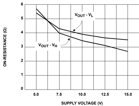
FIGURE 5. ON-RESISTANCE vs SUPPLY VOLTAGE, I_{OUT} = 200\text{mA} , T = +25^{\circ}\text{C} , V_{S+} = V_H , V_L = 0\text{V}
