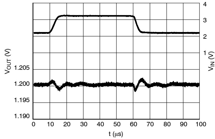
Figure 27. Line Transients, 1.2 V Version, t_R = t_F = 5 \mu\text{s} , I_{\text{OUT}} = 30 \text{ mA}
