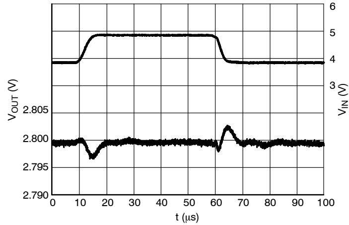
Figure 28. Line Transients, 2.8 V Version, t_R = t_F = 5 \mu\text{s} , I_{\text{OUT}} = 30 \text{ mA}
