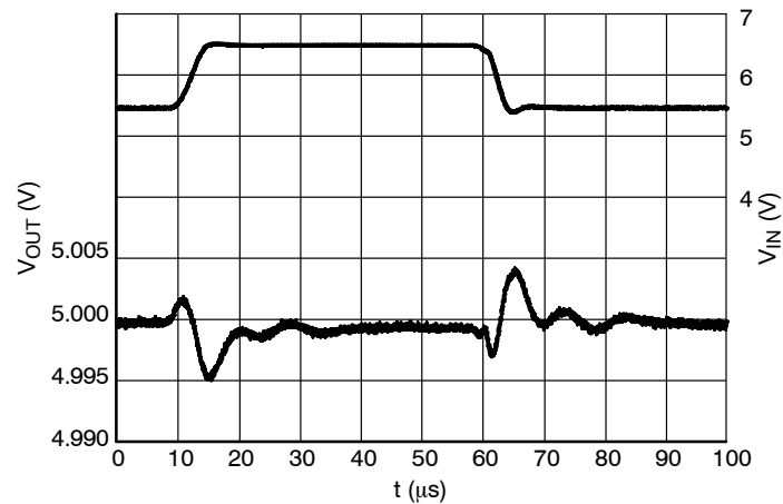
Figure 29. Line Transients, 5.0 V Version, t_R = t_F = 5 \mu\text{s} , I_{\text{OUT}} = 30 \text{ mA}
