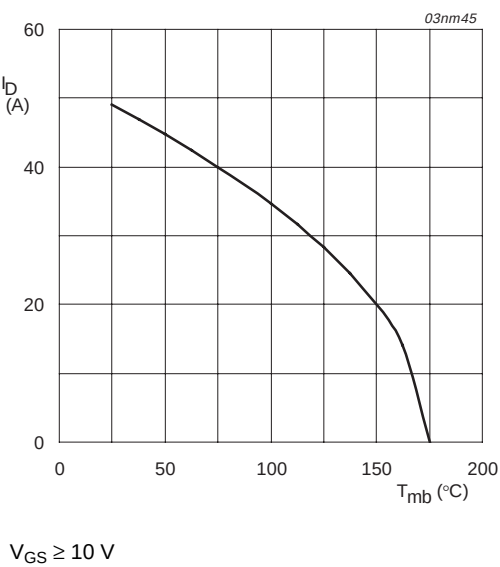
Fig 2. Continuous drain current as a function of mounting base temperature.
