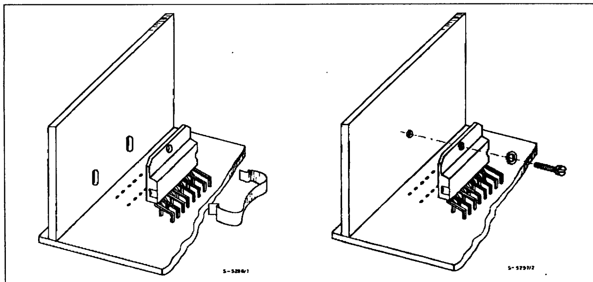
Figure 5 : Mounting Examples
