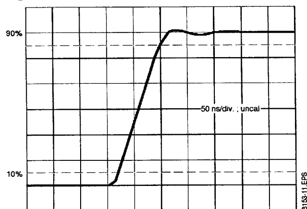
Figure 2 : Fall Time
