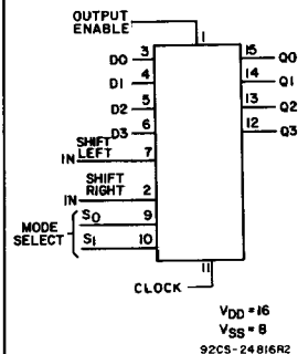
4-Bit Bidirectional Universal Shift Register CD40104B, CD40194B (File No. 1220)
