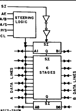
8-Stage Static Bidirectional Parallel/Serial Input/Output Bus Register
