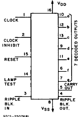
Decade Counter/Divider with 7-Segment Display Outputs and Ripple Blanking
