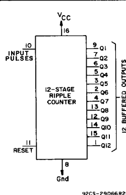
12-Stage Ripple-Carry Binary Counter/Divider
