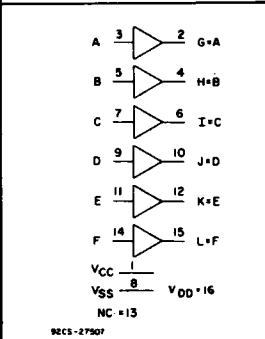
Hex Buffer/Converter Non-Inverting Type
