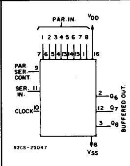
8-State Synchronous Shift Register with Parallel or Serial Input/Serial Output
