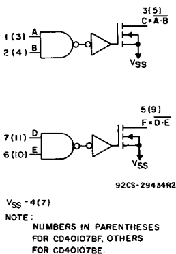
Dual 2-Input NAND Buffer/Driver CD40107B (File No. 1015)
