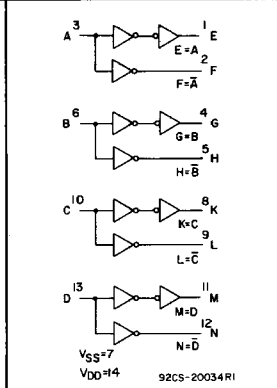
Quad True/Complement Buffer
