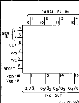
4-Stage Parallel In/Parallel Out Shift Register with J-K Serial Input and True/ Complement Outputs
