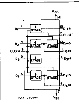
18-Stage Static Shift Register
