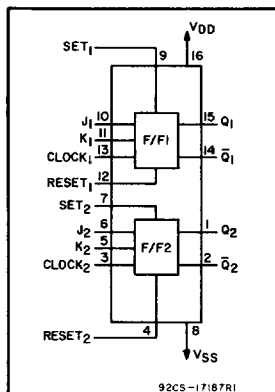
Dual J-K Master-Slave Flip-Flop with Set-Reset Capability
