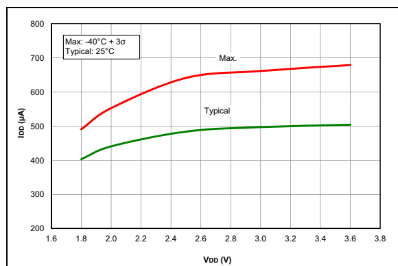
FIGURE 35-49: I_{PD} , Comparator, NP Mode ( CxSP = 1 ), PIC16LF1713/6 Only.
