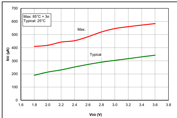
FIGURE 35-45: I_D , Op Amp, High GBWP Mode ( OPAxSP = 1 ), PIC16LF1713/6 Only.
