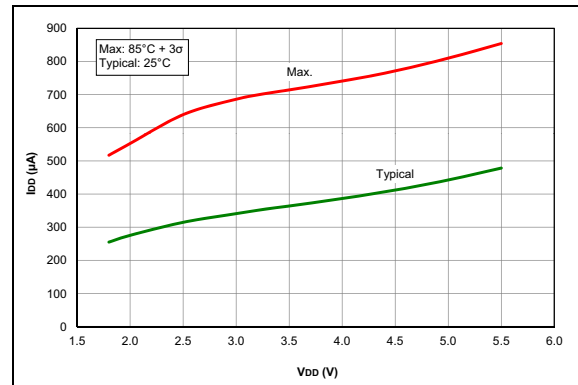
FIGURE 35-46: I_D , Op Amp, High GBWP Mode ( OPAxSP = 1 ), PIC16F1713/6 Only.
