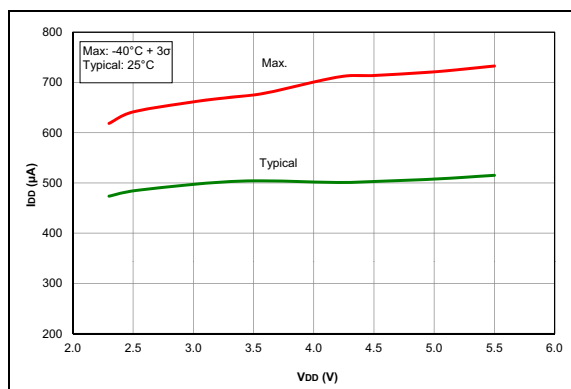
FIGURE 35-50: I_{PD} , Comparator, NP Mode ( CxSP = 1 ), PIC16F1713/6 Only.
