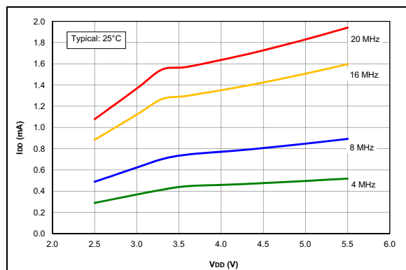
FIGURE 35-29: I_{DD} Typical, HS Oscillator, 25^\circ\text{C} , PIC16F1713/6 Only.
