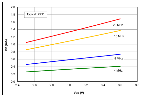
FIGURE 35-27: I_{DD} Typical, HS Oscillator, 25^\circ\text{C} , PIC16LF1713/6 Only.
