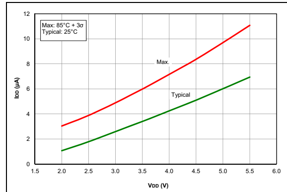
FIGURE 35-44: I_D , Timer1 Oscillator, F_{OSC} = 32\text{ kHz} , PIC16F1713/6 Only.
