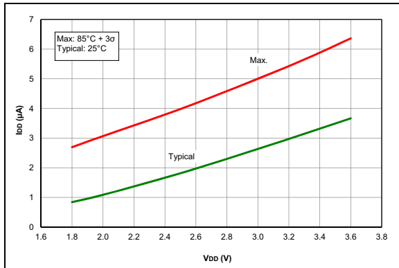
FIGURE 35-43: I_D , Timer1 Oscillator, F_{OSC} = 32\text{ kHz} , PIC16LF1713/6 Only.
