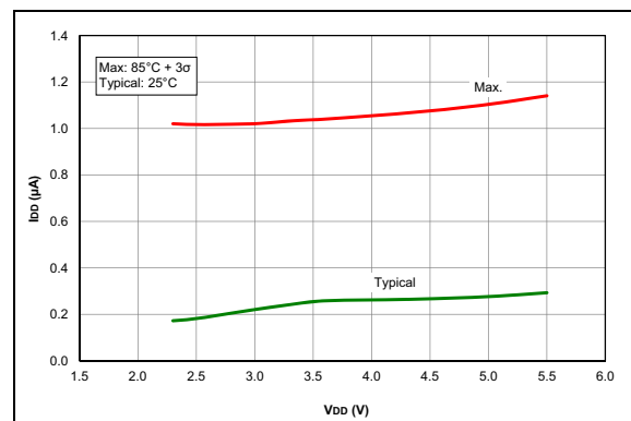
FIGURE 35-48: I_D , ADC Non-Converting, PIC16F1713/6 Only.
