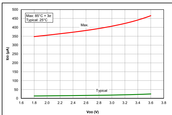
FIGURE 35-47: I_D , ADC Non-Converting, PIC16LF1713/6 Only.
