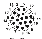
Plug, 17-pos.
