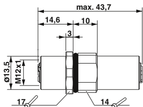
Control cabinet feed-through, socket to socket on both sides
