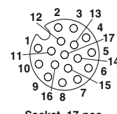
Socket, 17-pos.
