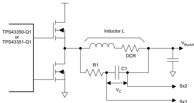
Figure 11. DCR Sensing Configuration
