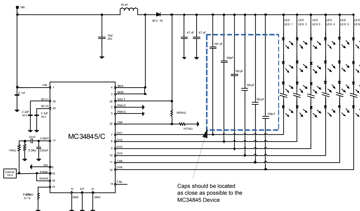
Figure 10. Typical Application Circuit for Single Wire Control, f_s = 600 \text{ KHz} ( V_{IN} = 9.0V , I_{LED}/\text{channel} = 20 \text{ mA/channel} , 10 \text{ LEDs/channel} , OVP = 35V , V_{PWM} = 3.3V )
