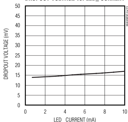
LED CURRENT-REGULATOR DROPOUT VOLTAGE vs. LED CURRENT
