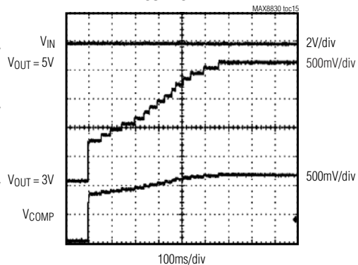
SOFT-START
