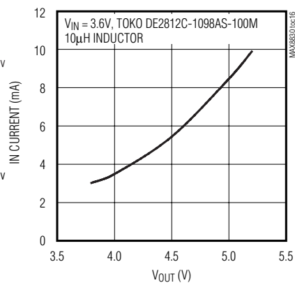
STEP-UP DC/DC IN SUPPLY CURRENT
