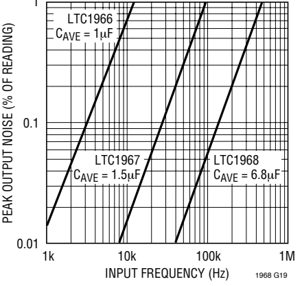
Output Noise vs Device
