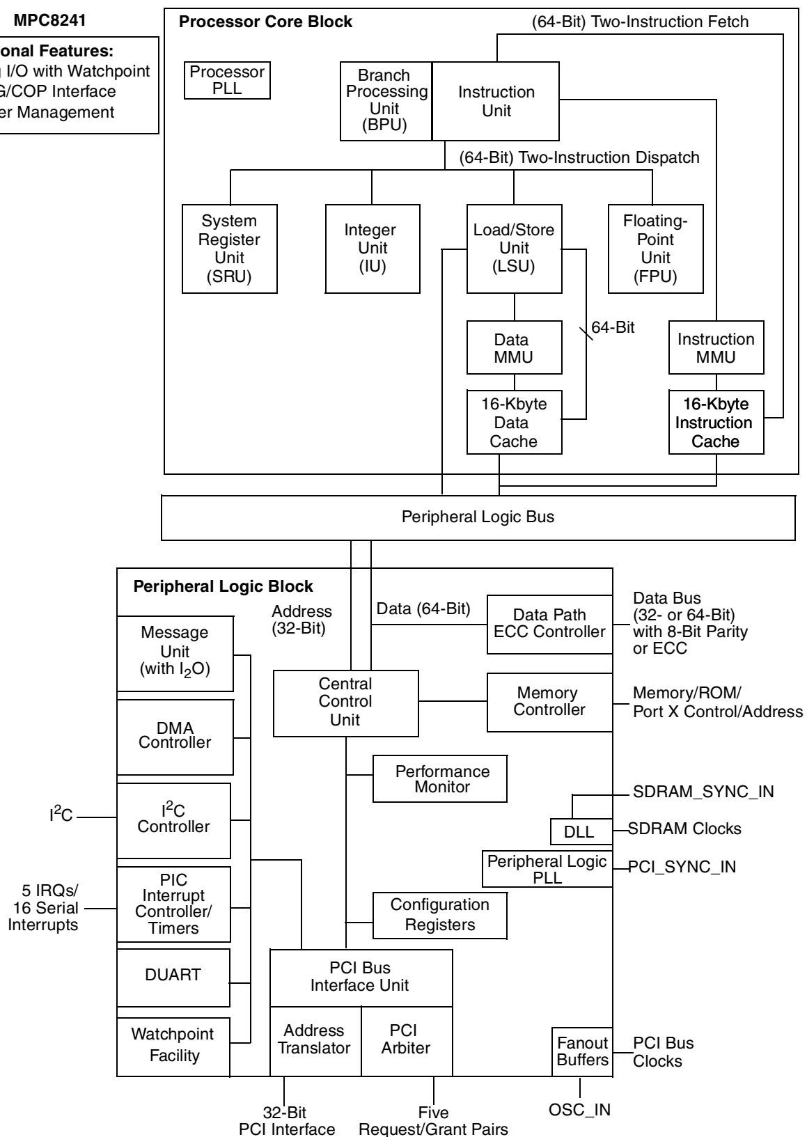
Figure 1. MPC8241 Block Diagram
