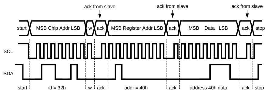
Figure 22. Write cycle (w = write; SDA = "0"), id = chip address = 32h for LP55231. This data pattern writes temperature information to the TEMPERATURE WRITE register (40h).
