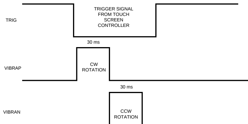
Figure 30. Control Waveform
