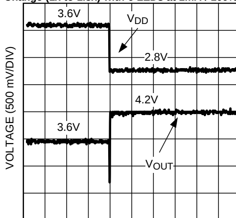
Line Transient and Charge Pump Automatic Gain Change (1x to 1.5x) with 6 LEDs at 1mA / 100% PWM
