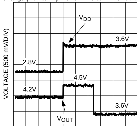
Line Transient and Charge Pump Automatic Gain Change (1.5x to 1x) with 6 LEDs at 1mA / 100% PWM
