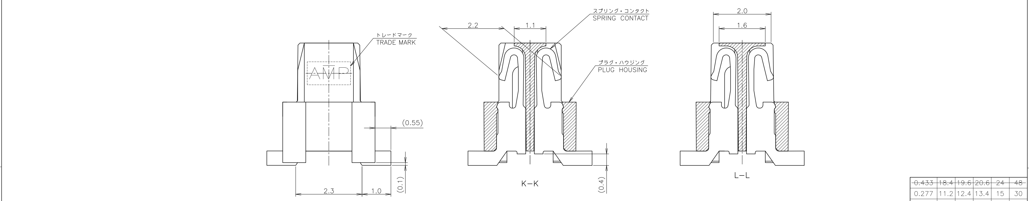
14, 18, 30 極 (n: 奇数) 14, 18, 30 POS (n: ODD NUMBER) 16, 20, 48 極 (n: 偶数) 16, 20, 48-POS (n: EVEN NUMBER) コネクタ外形 CONNECTOR EXTERNAL FORM 参考基板加工寸法 REFERENCE P.C. BOARD LAYOUT
