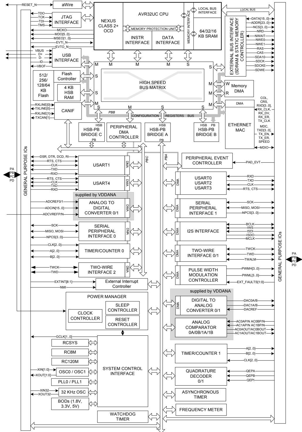
Figure 2-1. Block diagram
