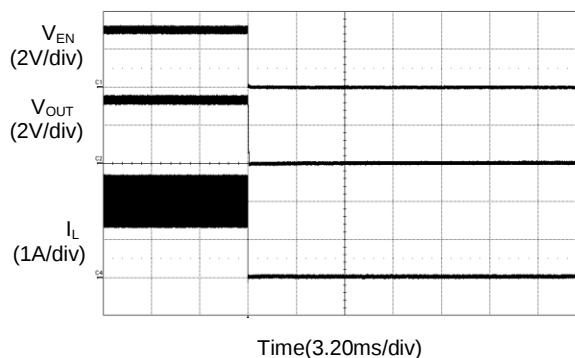
Power Off from EN ( I_{OUT}=2A )
