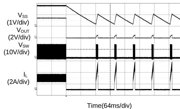
Short Circuit Protection Recovery ( I_{OUT}=2A )
