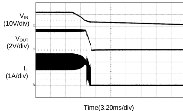
Power Off from VIN ( I_{OUT}=2A )
