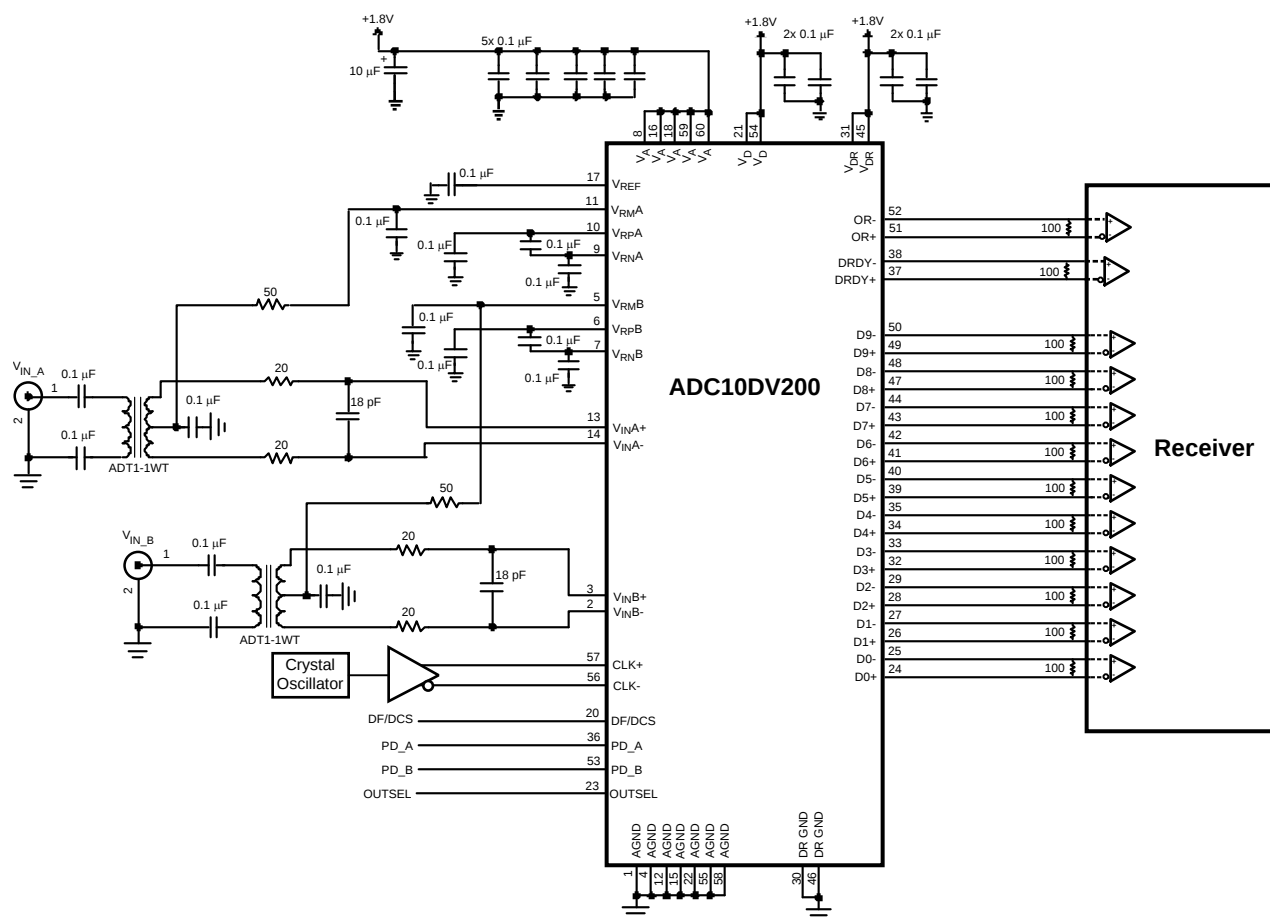
Figure 27. Application Circuit
