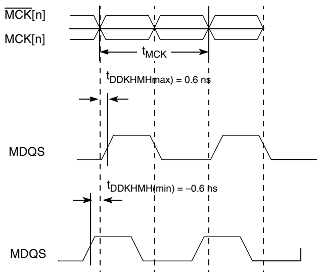
Figure 4. Timing Diagram for t_{\text{DDKMH}}
