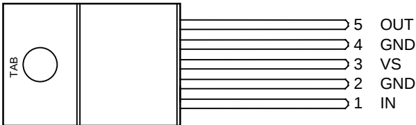
TO-220-5 (T)
