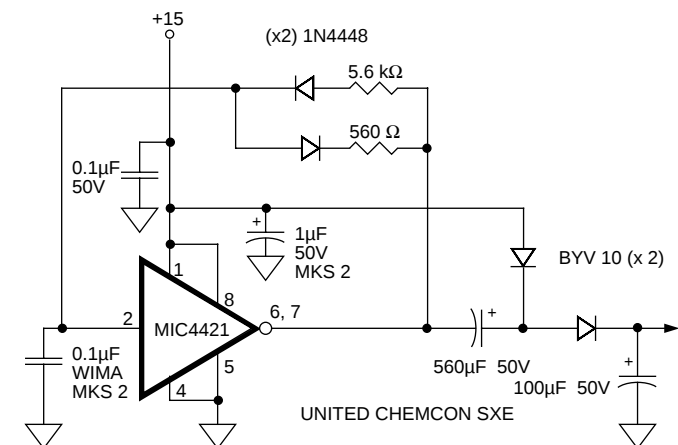
Figure 4. Self Contained Voltage Doubler
