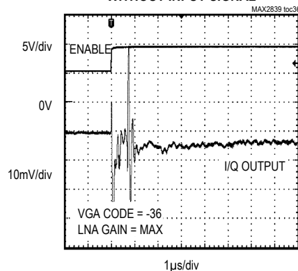
POWER-ON DC OFFSET CANCELLATION WITHOUT INPUT SIGNAL
