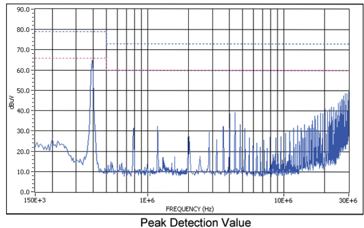
Graph 5. Conducted emissions performance, Positive Line, CISPR 22, Class A, 48 Vin, full load
