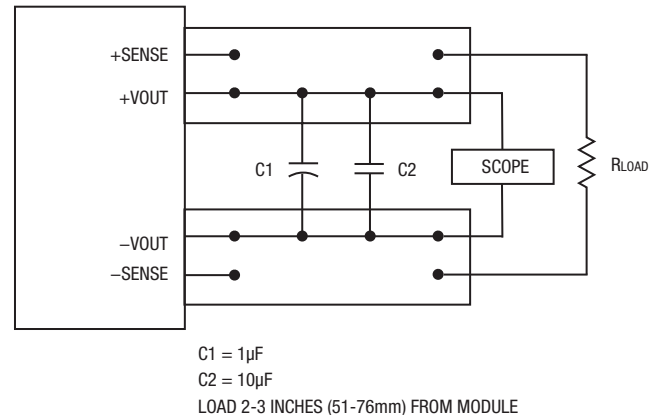
Figure 6. Measuring Output Ripple and Noise (PARD)
