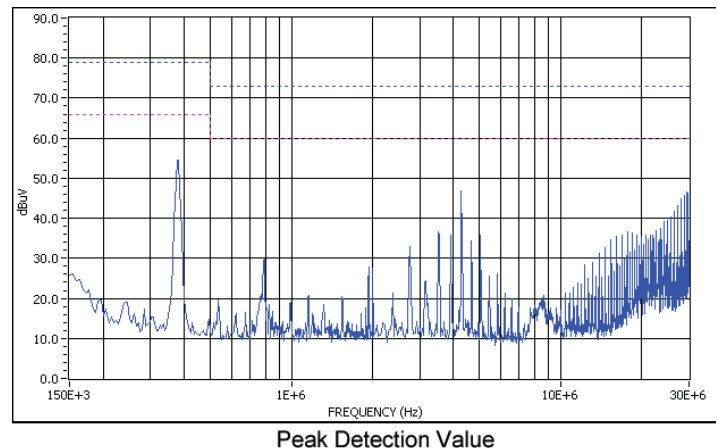
Graph 1. Conducted emissions performance, Positive Line, CISPR 22, Class A, 48 Vin, full load
