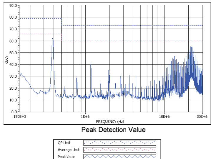
Graph 4. Conducted emissions performance, Negative Line, CISPR 22, Class A, 48 Vin, full load
