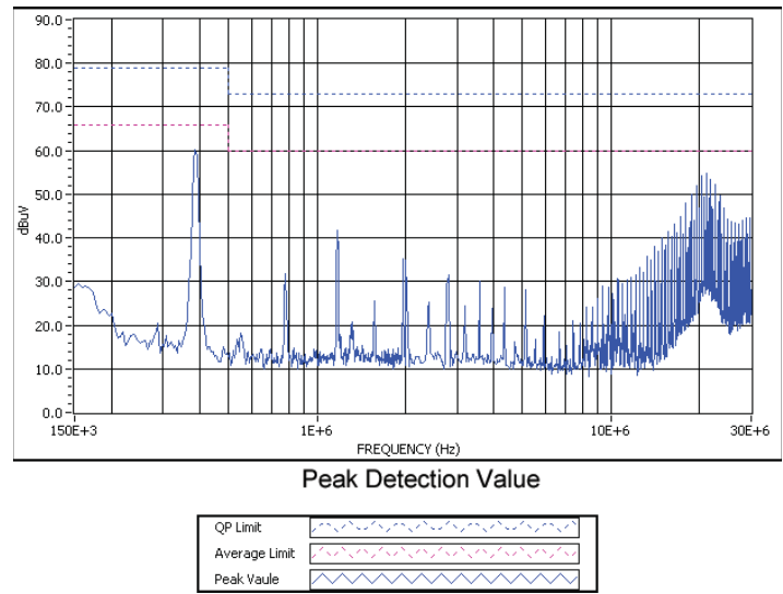
Graph 3. Conducted emissions performance, Positive Line, CISPR 22, Class A, 48 Vin, full load
