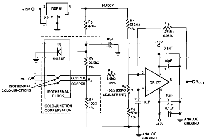
Figure 25. Thermocouple Amplifier with Cold Junction Compensation
