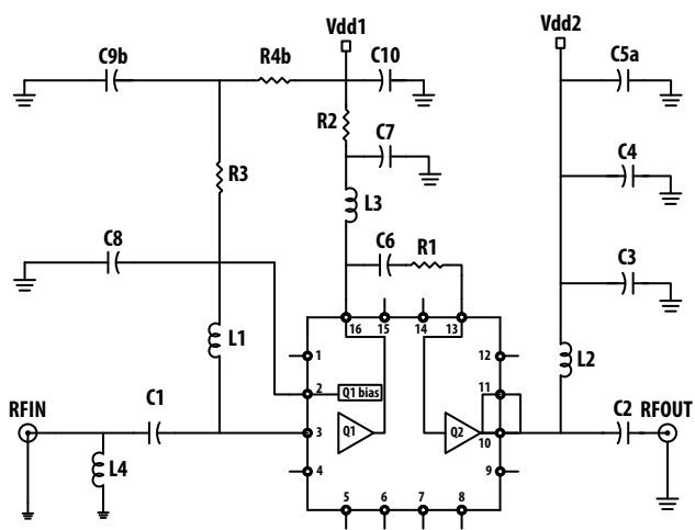
Figure 2 Simplified Schematic
