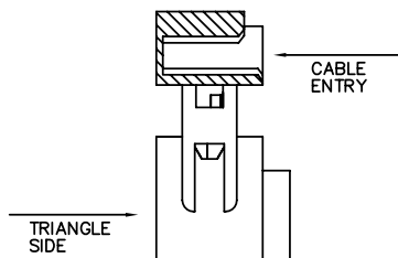
LEFT ASSY
