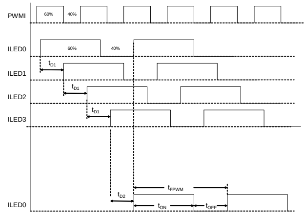
FIGURE 22. PHASE SHIFT WITH FIXED DELAY (4 CHANNELS)
