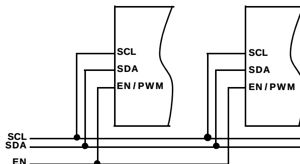
FIGURE 41. MULTIPLE DRIVERS OPERATION
