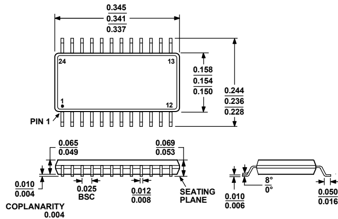
COMPLIANT TO JEDEC STANDARDS MO-137AE Figure 63. 24-Lead Shrink Small Outline Package [QSOP] (RQ-24) Dimensions shown in inches
