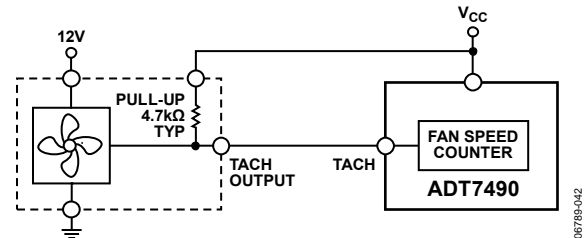
Figure 43. Fan with TACH Pull-Up to V_{CC}
