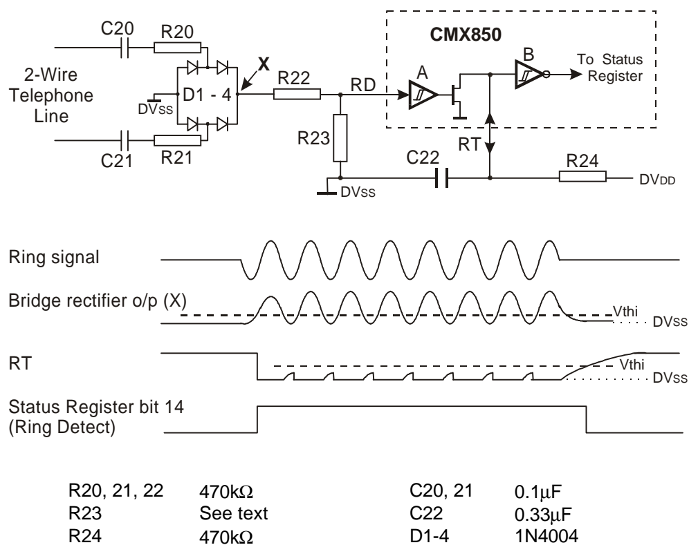
Figure 3 Ring Signal Detector Interface Circuit
