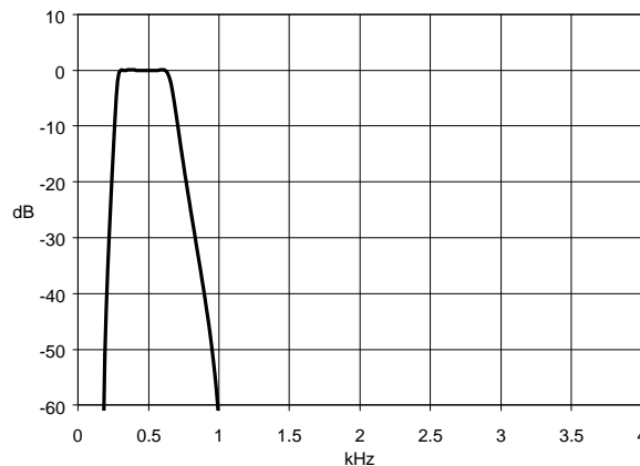
Figure 11a Response of the Call Progress Filter
