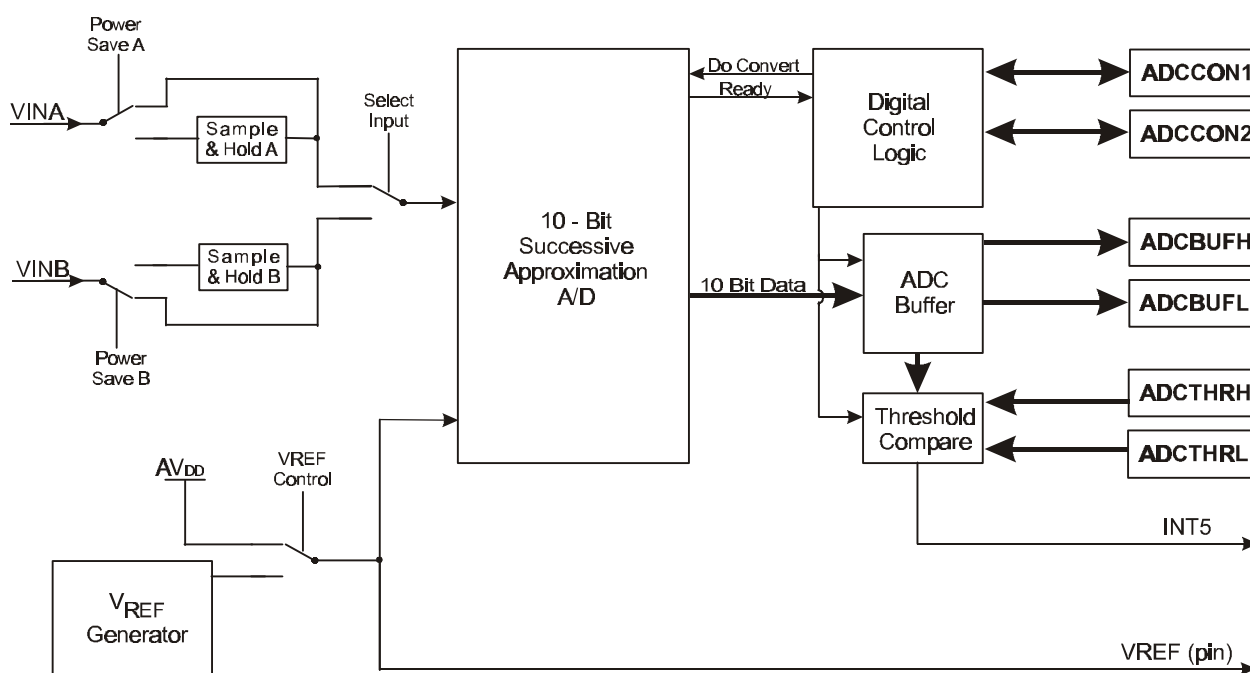
Figure 6 Analogue to Digital Converter Block Diagram
