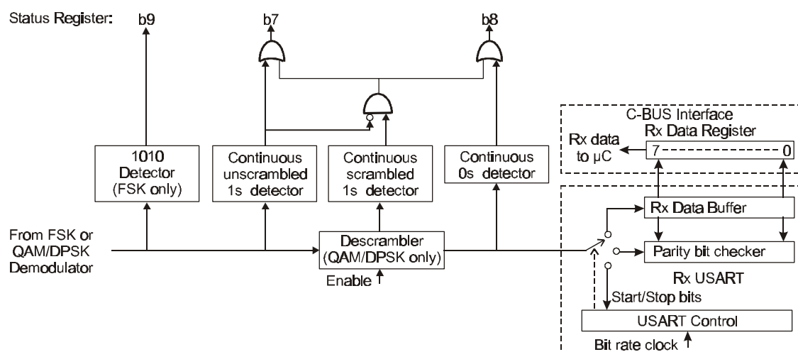
Figure 12a Rx Modem Data Paths
